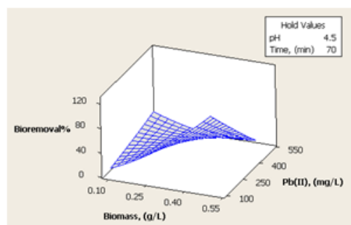
Fig. 3-3. Interaction of Pb (II) vs biomass
